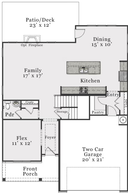
CLASSIC FIRST FLOOR
