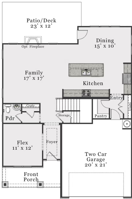
CRAFTSMAN FIRST FLOOR
