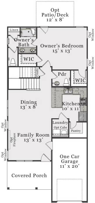
FIRST FLOOR C
