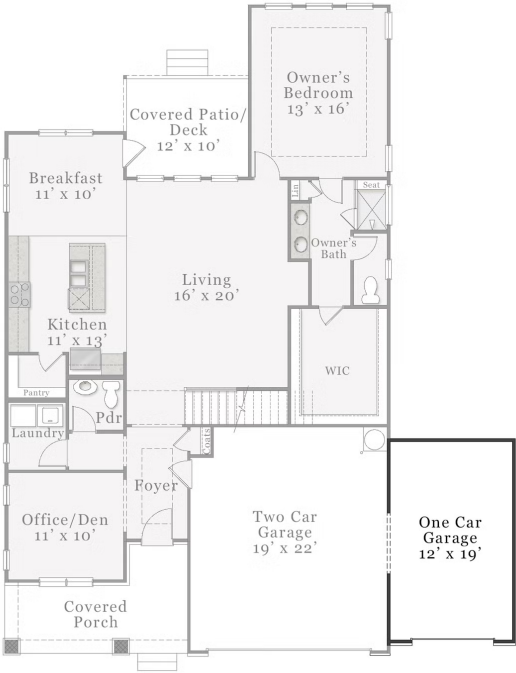
CRAFTSMAN & EUROPEAN OPTIONAL - 3RD CAR GARAGE
