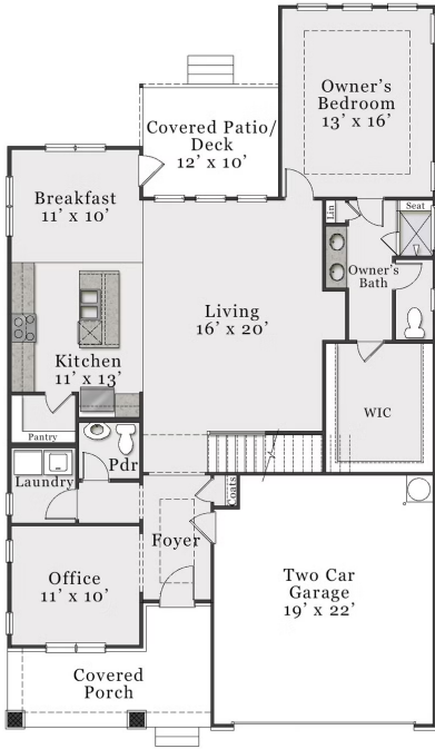
CRAFTSMAN FIRST FLOOR
