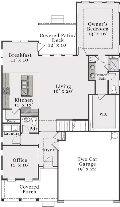
CLASSIC FIRST FLOOR
